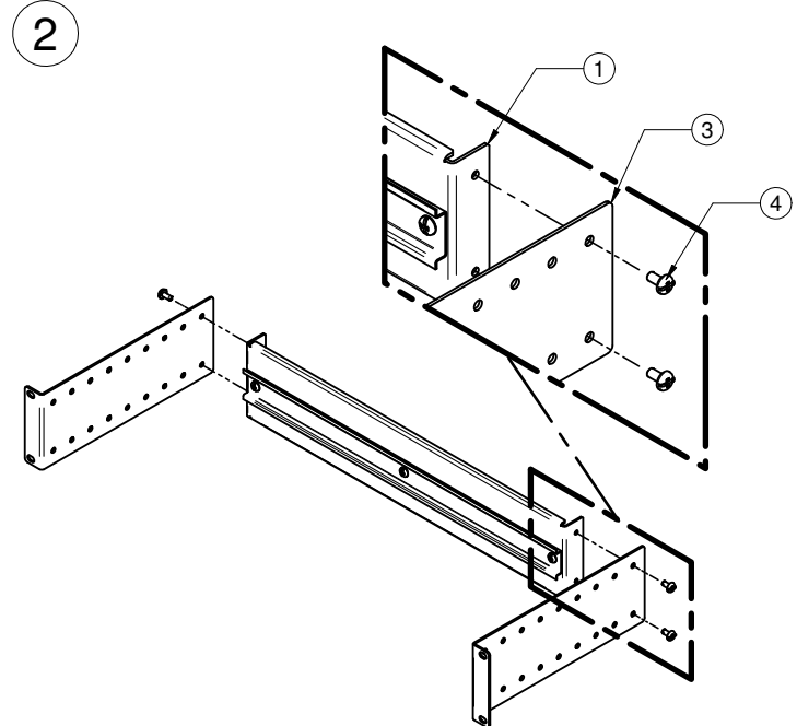
ITEM 3 RMHD - RAIL MTG FLANGES QTY 2
