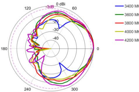
Azimuth (Top View): 3400 – 4200 MHz
