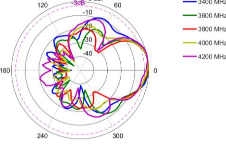
Elevation (Side View): 3400 – 4200 MHz
